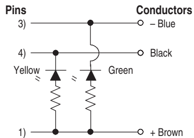
NPN (Sinking)
