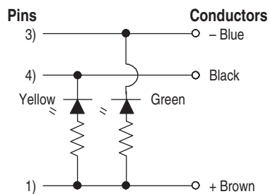
NPN (Sinking)
