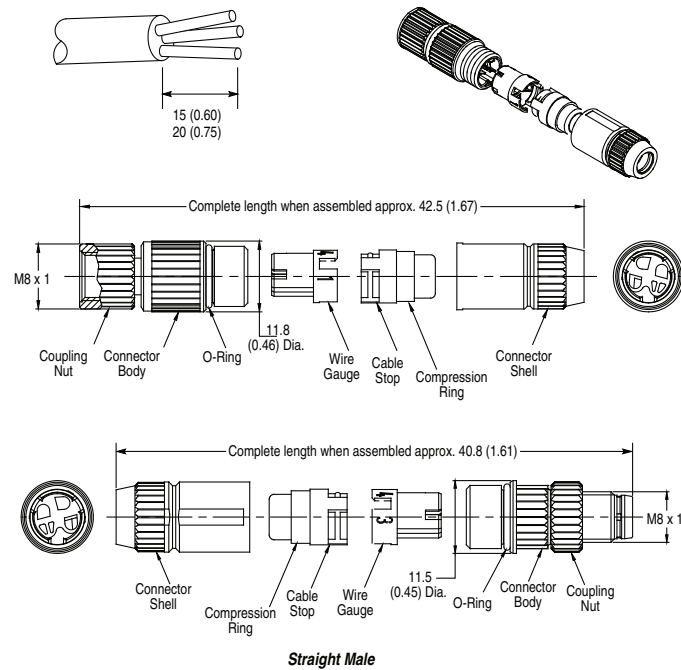
Straight Male
