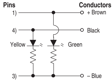
PNP (Sourcing)
