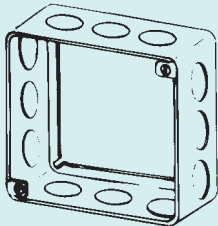
4SE-1/2 Extension Ring 1-1/2" Deep, Drawn Top: Two 8-32 screws Bottom: Two slide-on slots
