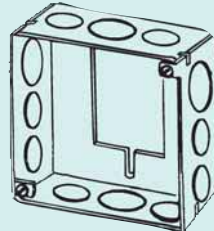
4SSBE-SPL Extension Ring 1-1/2" Deep, Welded Top: Two 8-32 screws Bottom: Cutout for switch or handy box
