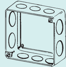
4SES Combo Extension-Thru-Ring 1-1/2" Deep, Drawn Top: Two 8-32 screws Bottom: Two 8-32 screws and two slide-on slots
