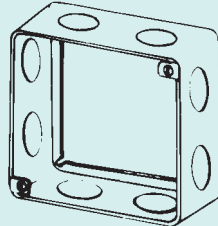
4SE-3/4 Extension Ring 1-1/2" Deep, Drawn Top: Two 8-32 screws Bottom: Two slide-on slots
