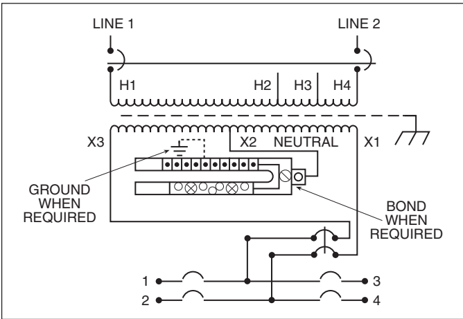
Wiring Diagram 1Ø 5-25 kVA
