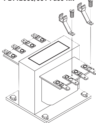
PL112600/601 Fuse Kit
