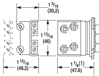
Shallow, PenTUFF™, and Logic Reed Contact Blocks 1-1/8 (28.6) Deep
