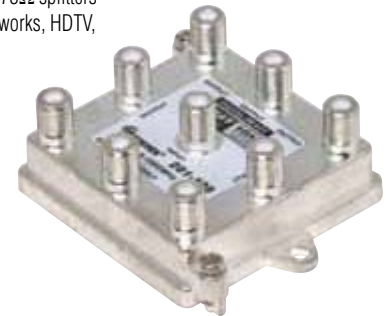
201-108 8-Way 1GHz 130dB RF Balanced Digital Splitter
