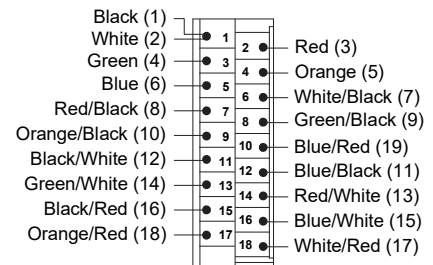
1492-CABLE 1CR (Red RTB)
