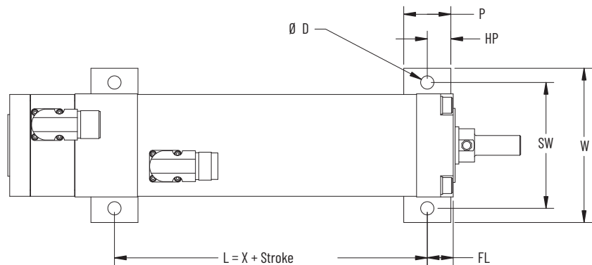
Piston Rod Cylinder Shown for Reference
