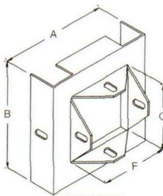
REDUCER Allows the reduction of a run of wireway to a smaller wireway size
