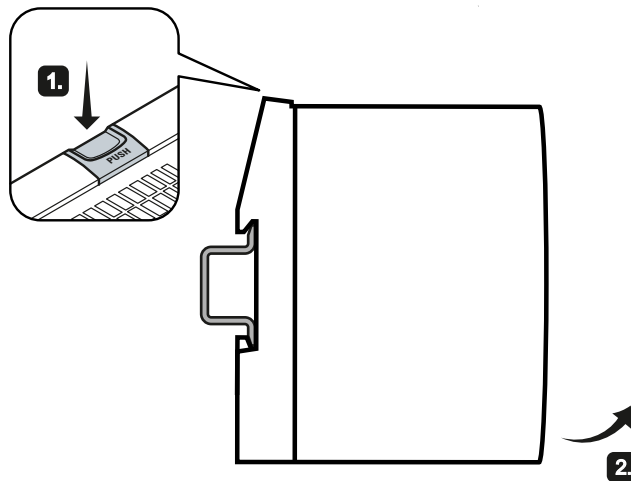
Figure 4-2 Removing from a DIN rail
