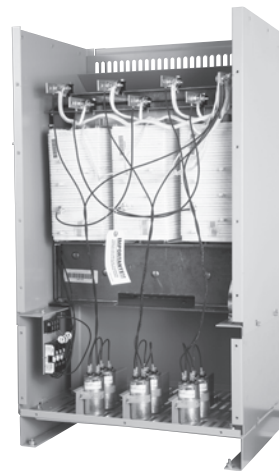
Guard II Transformer, (front panel removed)
