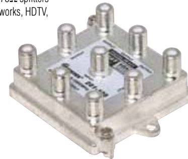
201-108 8-Way 1GHz 130dB RF Balanced Digital Splitter
