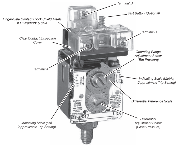
Figure 6 Trip and reset adjustment
