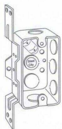
58361-V-1/2 "CV" bracket recessed 1/2"
